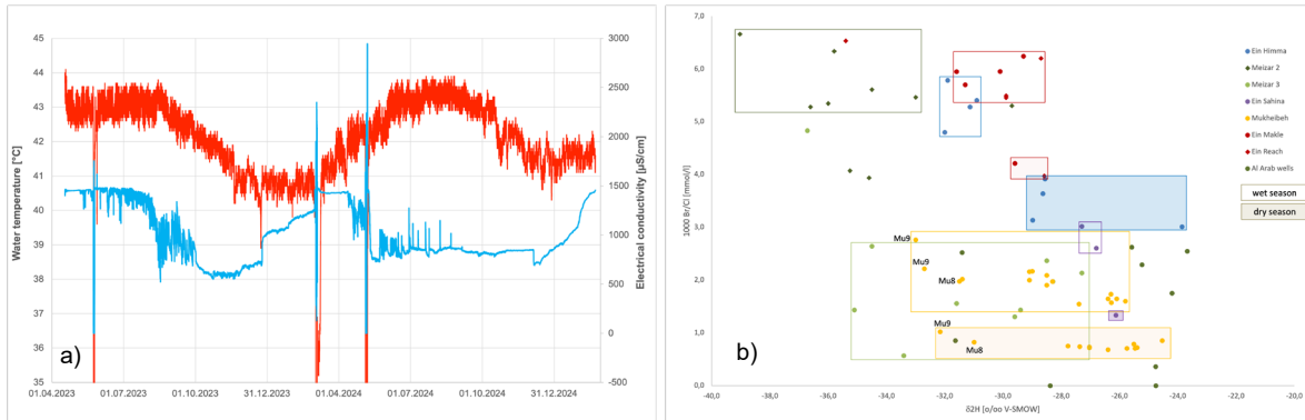
Fig. 2: show (a) temperature (red) and electrical conductivity (blue) in Himma Spring and (b) respective changes in all the groundwaters as for contributing of deep formation water, indicated by salinity tracer (Br/Cl) and Deuterium signatures during wet and dry seasons, respectively.
