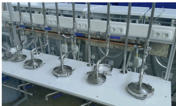
Washing tests are carried out to measure the extent of textile microplastic emissions. The picture shows the filter system and washing machines at the Niederrhein University of Applied Sciences.
